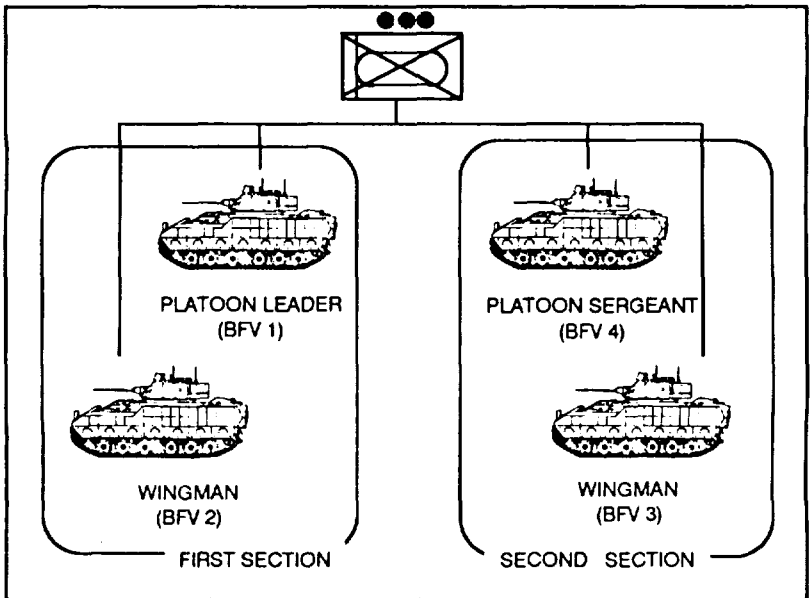
Figure 2-73. M2 platoon.
